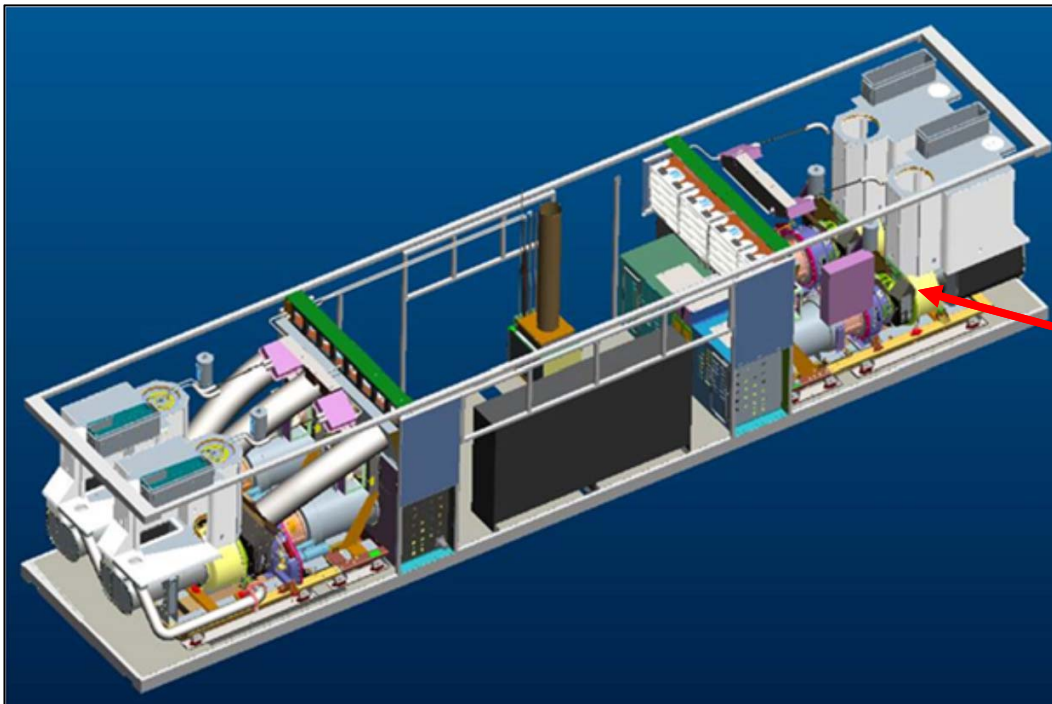
FLEX TURBINE™ GT333S modular drive train
