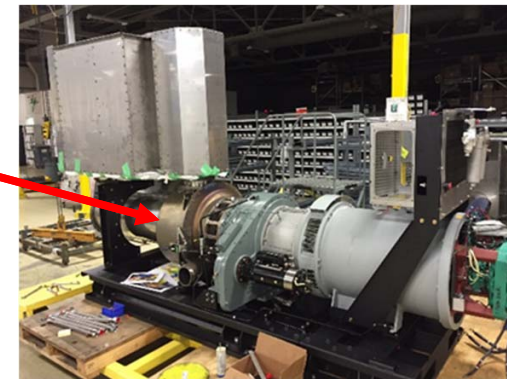
FLEX TURBINE™ GT333S modular drive train
